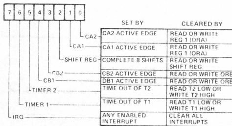
Figure 25. Interrupt Flag Register (IFR)
