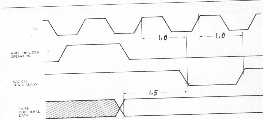
Figure 5c. CA2, CB2 Timing for Write Handshake, Pulse Mode
