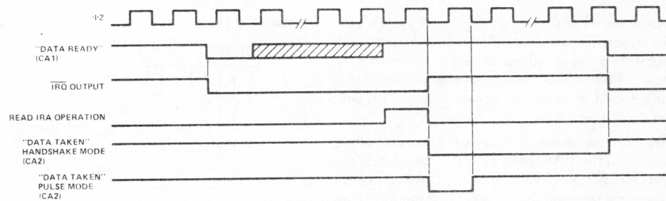
Figure 12. Read Handshake Timing (Port A, Only)
